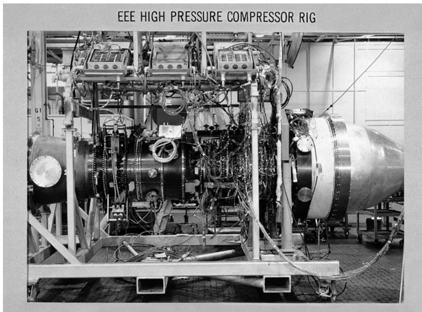
Energy Efficient High Pressure Compressor Rig (April 10, 1984). (NASA Glenn Research Center [NASA GRC].)
