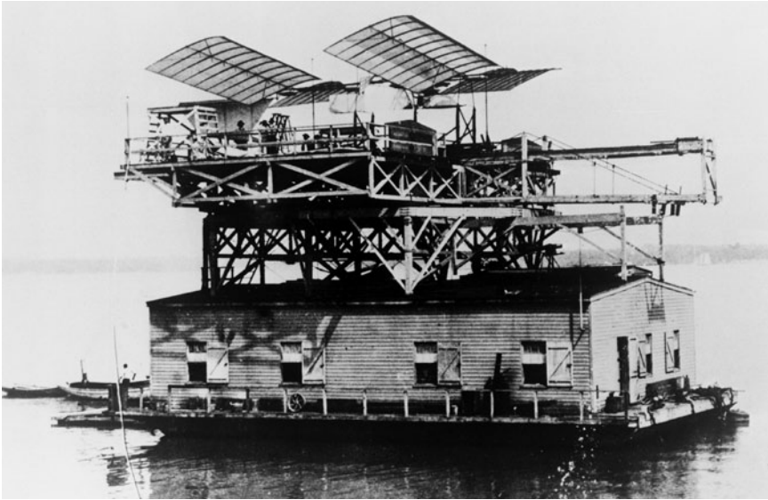
The Langley aerodrome (December 8, 1903). After this photo was taken, the project ended in failure when it fell into the Potomac River. (NASA Langley Research Center [NASA LaRC].)
