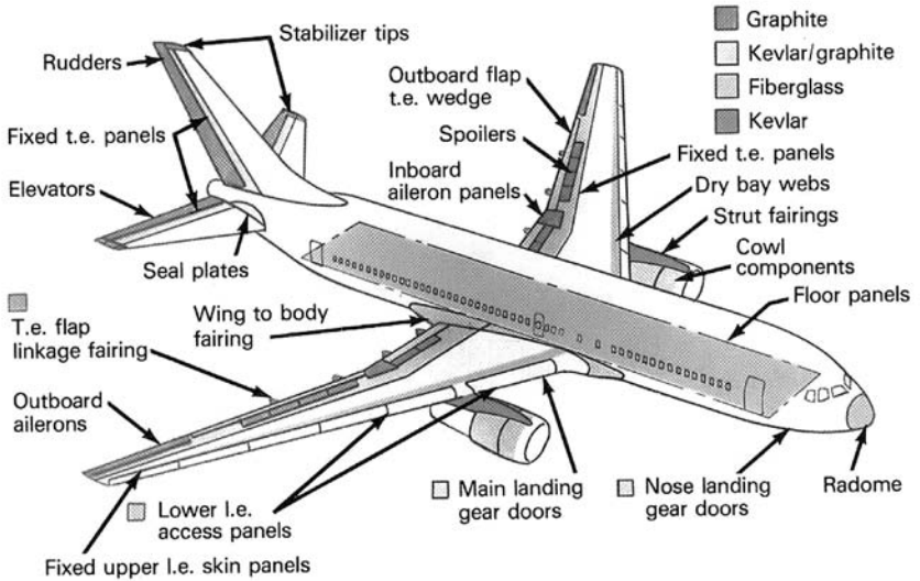
The above graphic demonstrates the composite components of the Boeing 767. Courtesy of Joseph Chambers.
