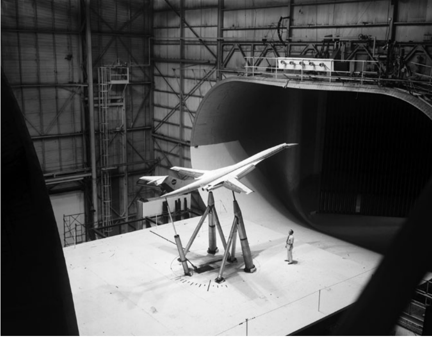
The end of the first SST era (July 1, 1973). A model of the Supersonic Transport (SST) variable sweep version, with wings in the low-speed position, mounted prior to tests in the Full Scale Wind Tunnel. (NASA Langley Research Center [NASA LaRC].)
