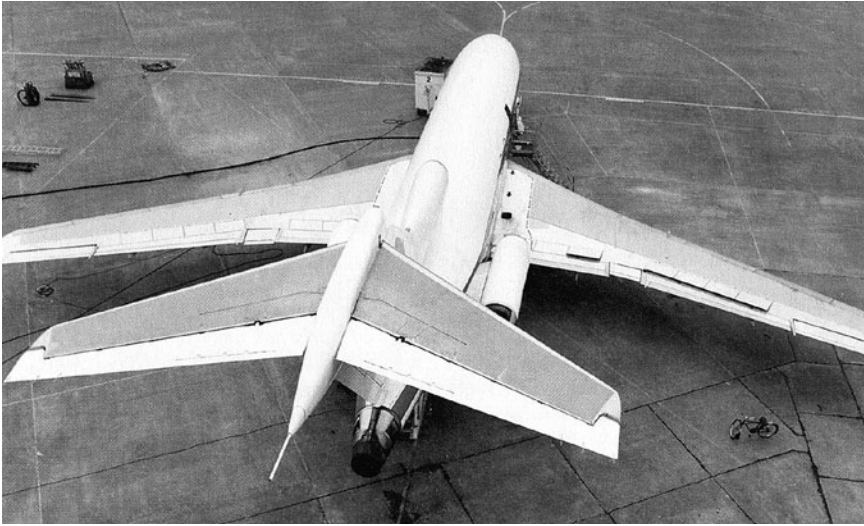
Composite elevators in flight evaluations on Boeing 727 during ACEE program. Courtesy of Joseph Chambers.
